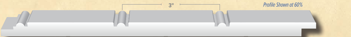
3" STANDARD BEAD (9" FACE) 1 LINEAL FT = .75 SQ FT – ORDER IN 5 PIECE INCREMENTS
