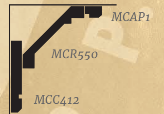
MCR550 MCAP1, MCC412
