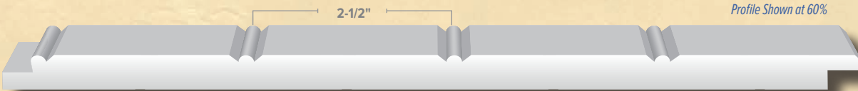
2-1/2" V-BEAD (10.104" FACE) 1 LINEAL FT = .842 SQ FT – ORDER IN 4 PIECE INCREMENTS
