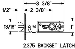
2.375 BACKSET LATCH
