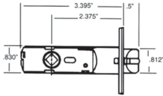
2.375" BACKSET LATCH
