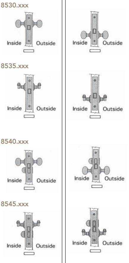
(Normal Installation) (Reverse Installation, order opposite door handing)
