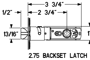
2.75 BACKSET LATCH
