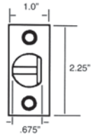
Standard Box Strike (T-Strike)
