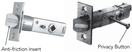
1" WIDE FACEPLATE
